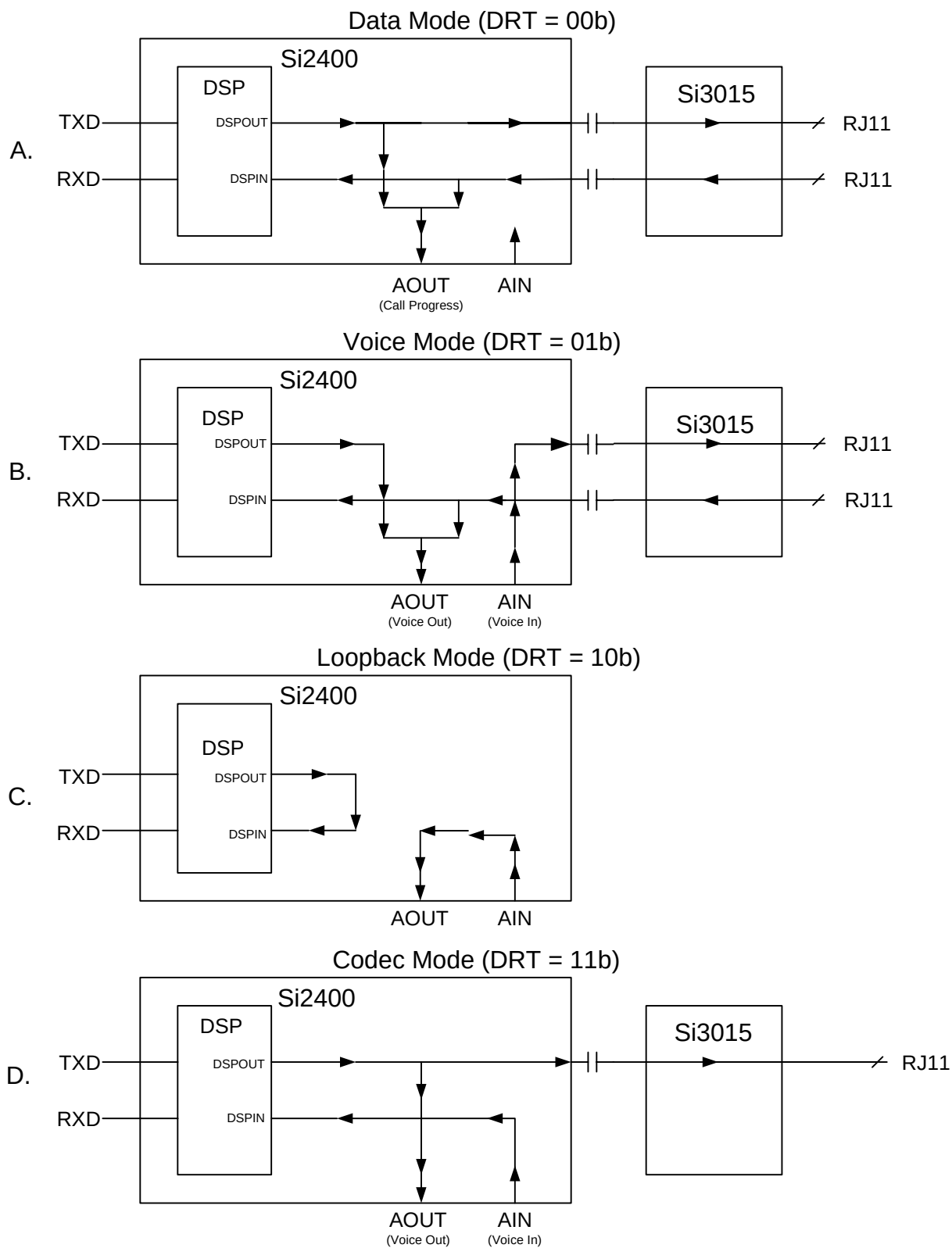
Figure 10. Signal Routing
